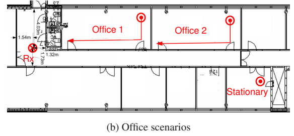
Fig. 1. Measured scenarios: (a) Left: Cafeteria (room length \sim 9 m), metal tables and chairs, some people sitting at the tables; (a) Right: Laboratory environment, Rx in the Cafeteria; (b) Office rooms (room width \sim 4 m), amply furnished
