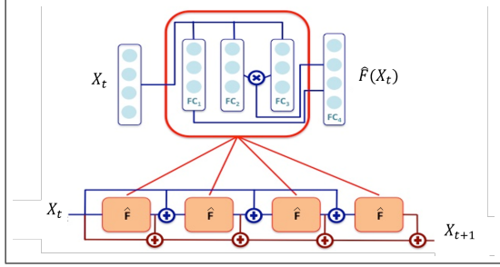
Fig. 1: Proposed bilinear residual architecture for the representation of a dynamical system represented by (1). We illustrate an architecture associated with a 4 th -order Runge-Kutta-like numerical integration for an elementary time-step dt = 1 . It involves a four-layer residual neural net with an elementary network \hat{F} repeated four times. The output of this elementary network involves a fully-connected layer FC_4 whose inputs are the concatenation of the output of the fully-connected layer FC_1 and the element-wise product between the outputs of fully-connected layers FC_2 and FC_3 .
