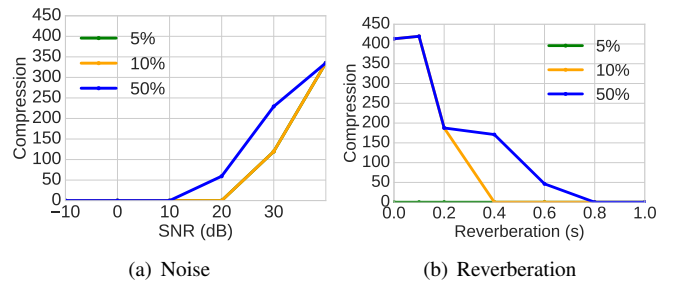
Fig. 4. Maximum compression when the TDOA relative error \leq 5\% , 10\% , 50\% for a source located at DOA 45^\circ for different values of noise and reverberation. In 4(a), white Gaussian noise of -10 dB, 0 dB, 10 dB, 20 dB, 30 dB and 40 dB signal-to-noise ratio per sample was added to the original signal. For 5\% and 10\% , the compression ratios are identical, therefore we can only visualize a single line. In 4(b), we simulated reverberation values of T_{60} = 0.1, 0.2, 0.3, 0.4, 0.5, 0.6, 0.7, 0.8, 0.9, 1 seconds.
