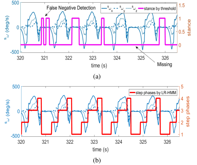
Figure 2: Step segmentation, jump 1 represents the stance phase. Stance detection by (a) a threshold method, where false negative detection and missing ones can be observed. (b) the proposed LR-HMM method.
