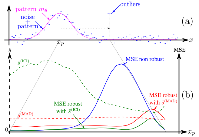
Fig. 3. Estimation of the position of a pattern by a robust approach using the MAD and the proposed ICI rule. Evolution of \hat{s} and MSE are respectively in dash and solid lines.
