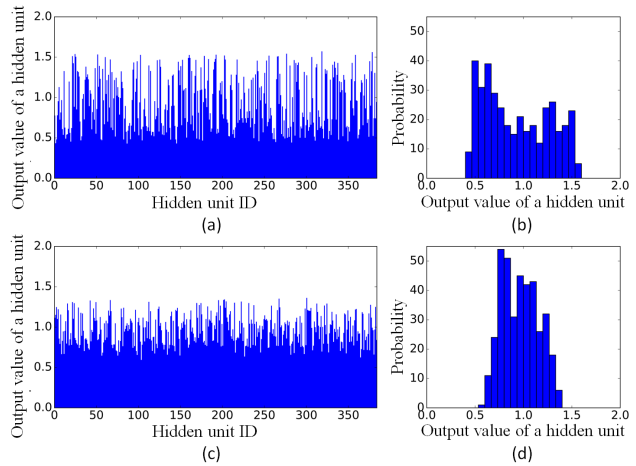
Fig. 3. (a), (c) are the output values of hidden units added to the fc4 layer. The vertical axis is the output value of hidden unit [0-2]. The horizontal axis is the hidden unit ID in fc5 layer. (b), (d) are their histograms. Upper is user ID3 and lower is user ID4.
