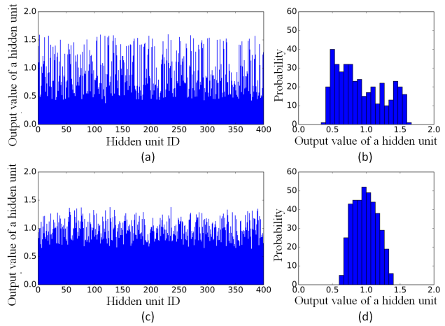
Fig. 4. (a), (c) are the output values of hidden units added to the fc5 layer. (b), (d) are its histogram. Upper is user ID3 and lower is user ID4.
