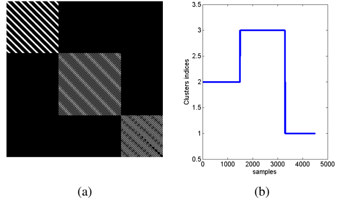
Fig. 2: (a) matrix of sparse coefficients, (b) clusters indices
