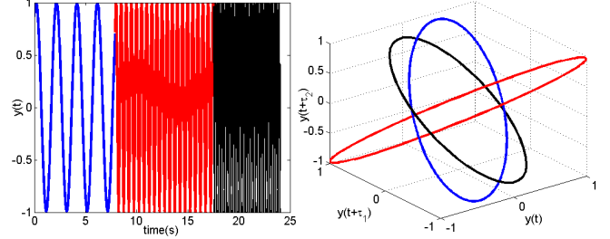
Fig. 1: left: y(t) with constant amplitude and 3 different frequencies in different colors. Right: delay embedding Y_3(t)
