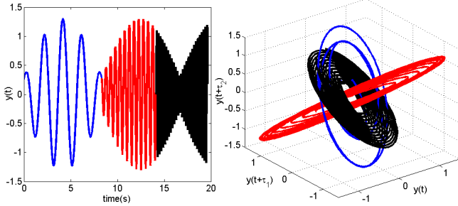
Fig. 3: left: y(t) with time varying amplitude and 3 different frequencies. Right: delay embedding
