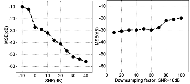
Fig. 5: left: Mean square frequency estimation error versus SNR, right: MSE versus downsampling factor for SNR = 10dB
