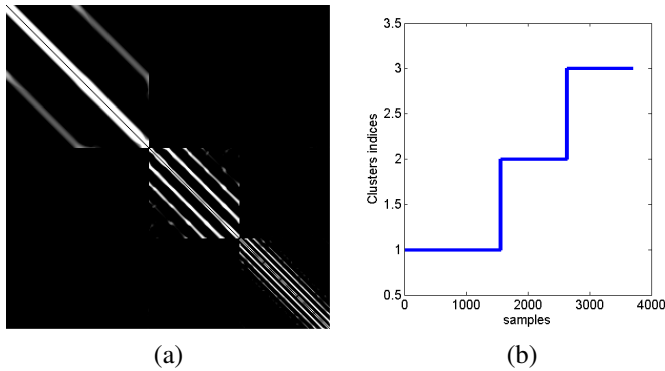
Fig. 4: (a) matrix of sparse coefficients, (b) clusters indices
