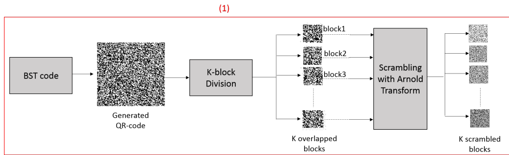
Fig. 2. The watermark preprocessing step
