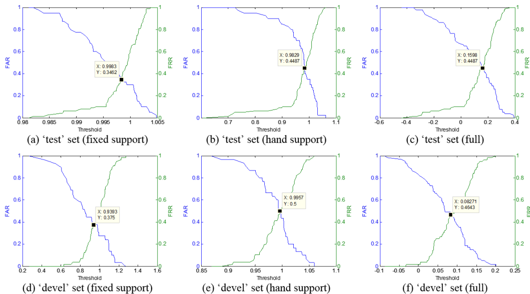
Fig. 4. ROC curves for employing the HSFV based spoofing detection on different combinations of the experimental datasets.
