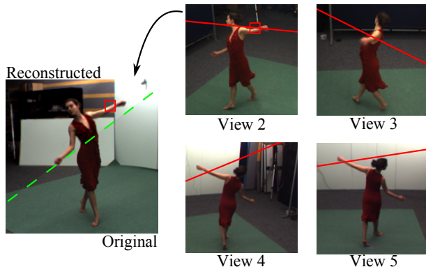
Fig. 1. Patch-based reconstruction by choosing the best match on epipolar lines in the other available views. The left image of this figure shows the reconstruction (top-left half) along with the original image (bottom-right part of the image).
