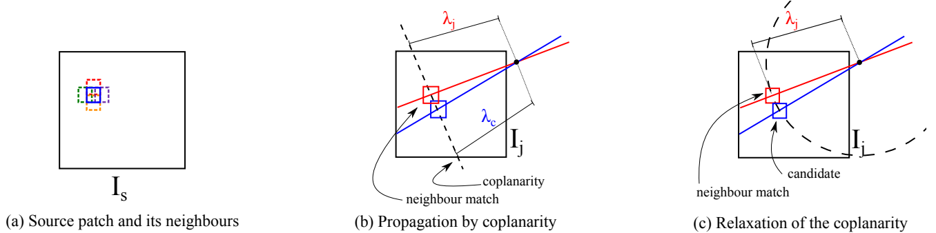
Fig. 2. The proposed mechanism for multi-view propagation. (b) presents a generalization for wide-baseline multi-view cases of the 2D local coherency by coplanarity propagation to determine the candidate patch (blue) from the neighbor patch (red). Then we propagate the position parameter \lambda_j between neighbor patches with circular propagation , as shown in (c).
