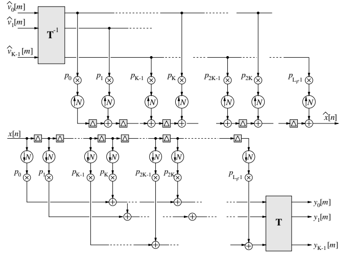
Fig. 6. Polyphase implementation of (top) transmitter and (bottom) receiver filter bank based multicarrier modulation.
