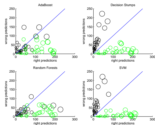
Figure 6: Scatter plot of the prediction made by different learning methods on the total patches of each painting.
