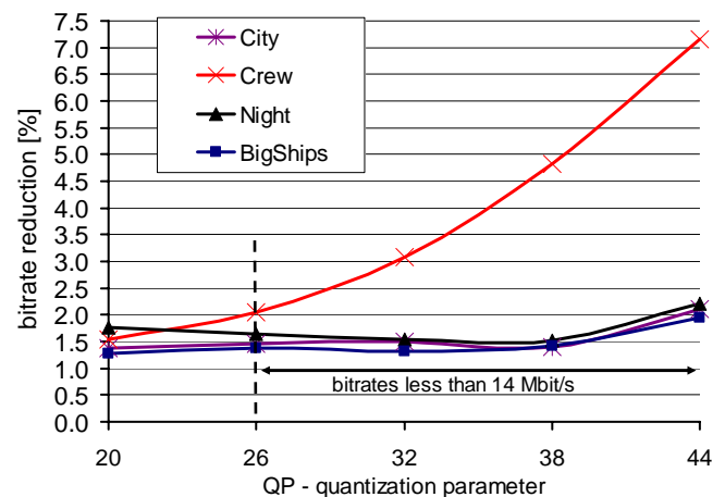
Figure 6 – Bitrate reduction using the improved AVC encoder compared to the original AVC encoder.
