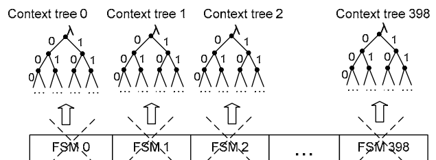
Figure 4 – Context trees in improved context modeler.
