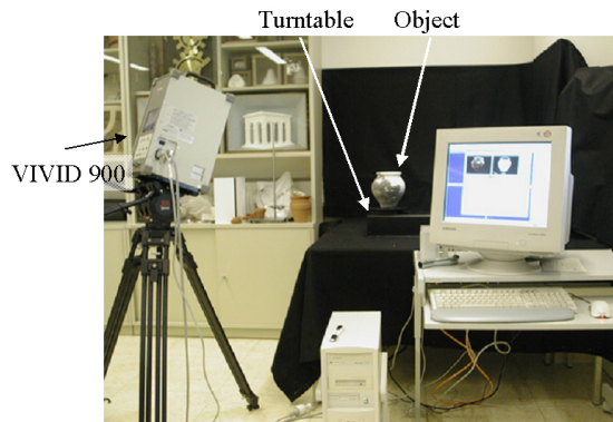
Figure 1: The Minolta VIVID 900 scanner.
