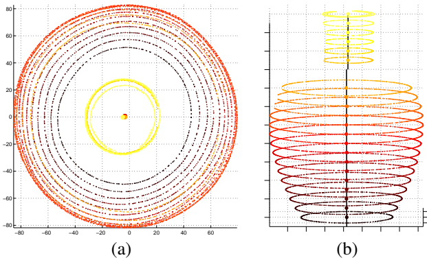
Figure 4: (a) Top-view and (b) side-view of the horizontal cross-sections - the level of gray corresponds to the height. The axis of rotation for the lower and upper part is shown as black line, defined by the centers of the concentric circles (shown as dots).
