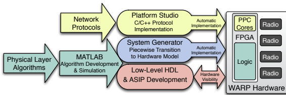
Figure 4: WARP Design Flows
