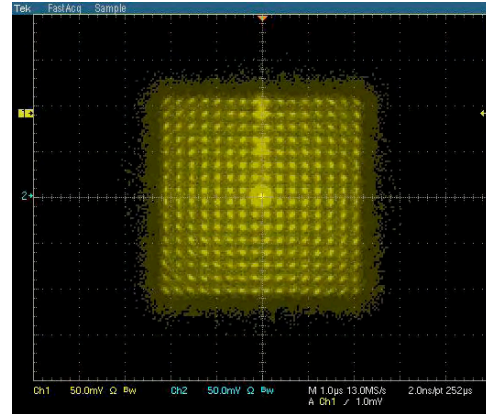
Figure 5: 256-QAM constellation viewed at the output of our OFDM transceiver, running in real time in the FPGA.
