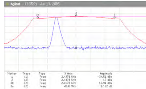
Figure 3: Spectrum analyzer view of an RF signal transmitted by our custom radio board.
