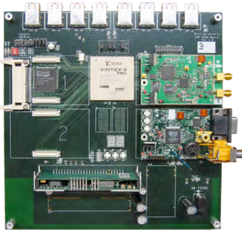
Figure 2: First revision of the platform's custom hardware, including the Virtex-II Pro FPGA board, radio daughtercard (top right) and video daughtercard (bottom right).
