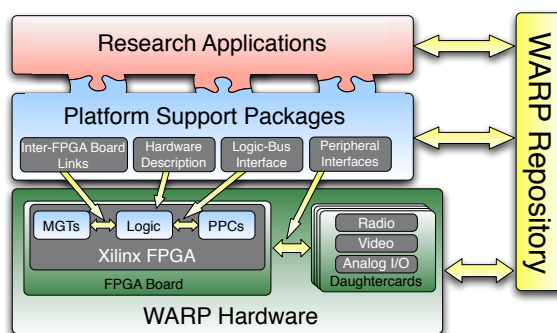
Figure 1: Components of the platform design
