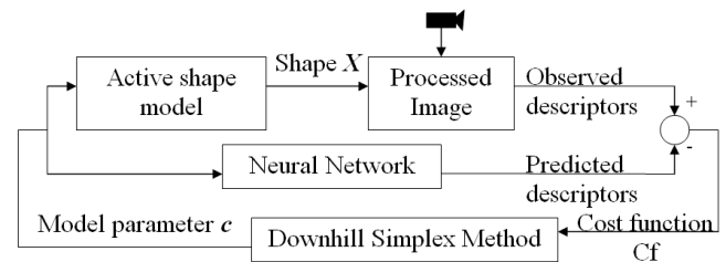
Figure 6 - Principle of segmentation of mouth segmentation with local descriptors
