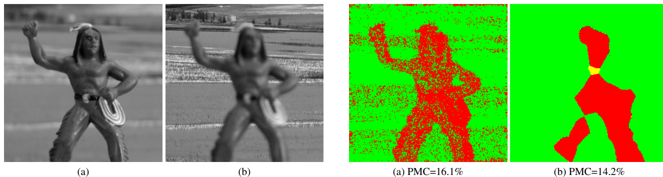
Figure 3: Real two-plane scenario: Two 256 \times 256 real images acquired with different focus points; (a) Indian in focus, (b) background in focus.
