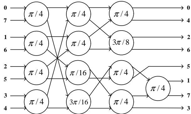
Figure 4: Pure Cordic based Loeffler DCT architecture.
