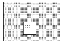
(b) subsampling
